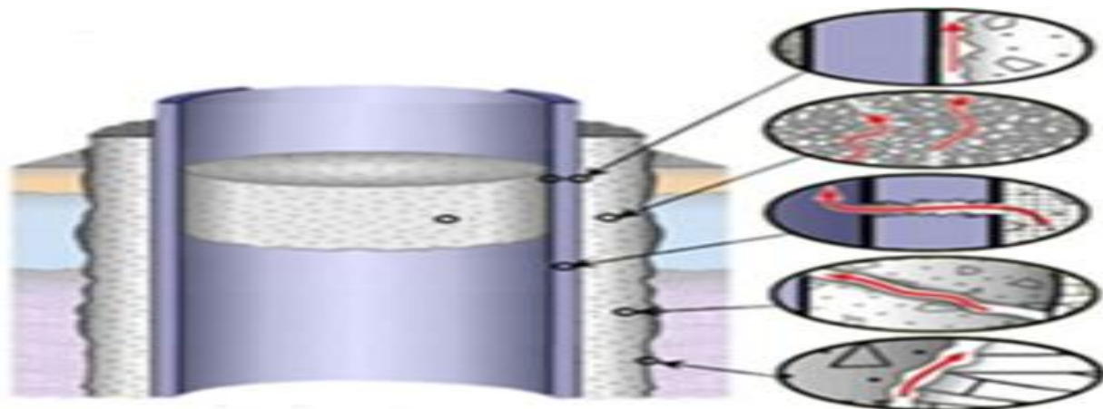
Figure 3 Interface flows [6]
